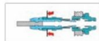
Connector is disengaged by a single axial pull on the outer release sleeve
