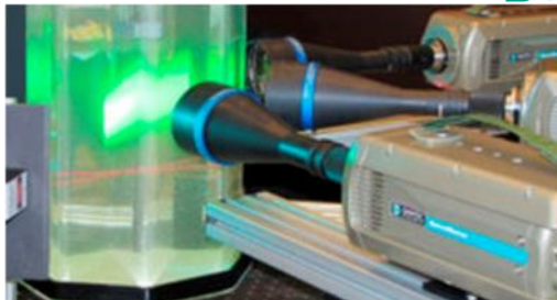
DANTEC PIV system for velocity, turbulence measurement and flow visualization
